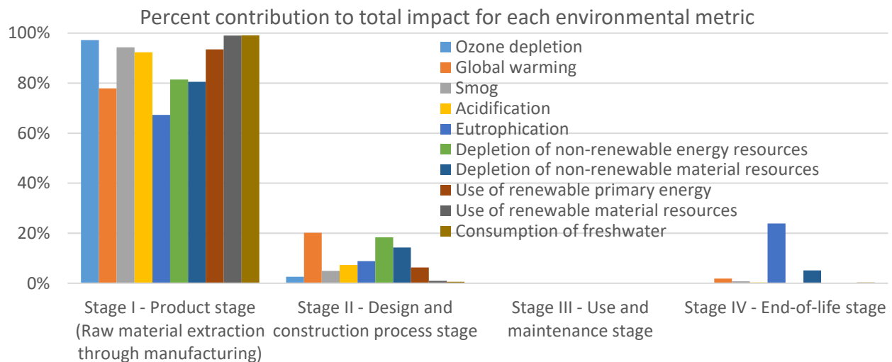
Figure 3 - Graphical impacts for the average PPG COPPER ARMOR Interior Paint product showing % contribution by life cycle stage
